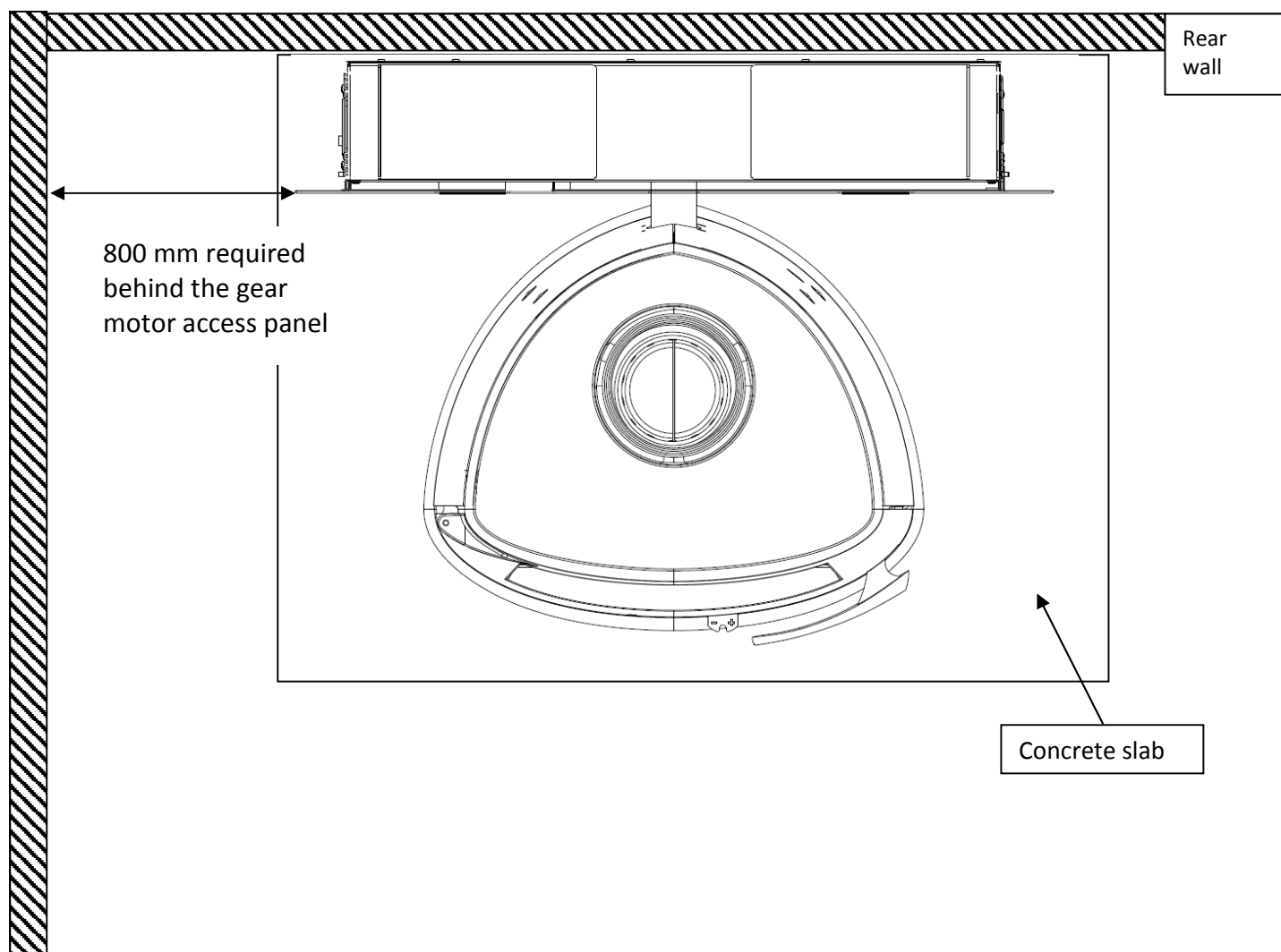
FLOOR PLAN OF STOVE INSTALLATION
